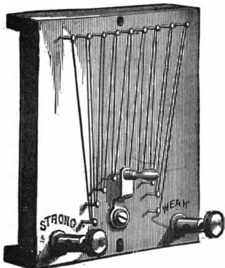
FIG. 41. RESISTANCE BOARD.
