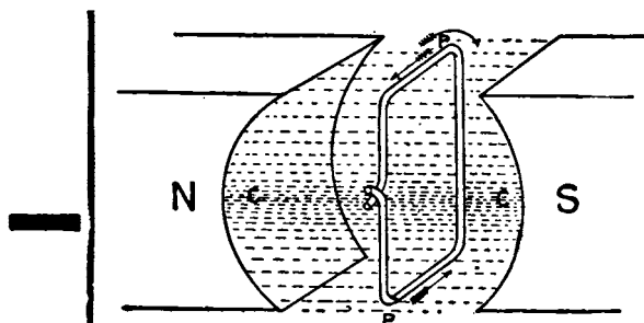
FIG. 11. DIAGRAM SHOWING HOW THE LINES OF MAGNETIC FORCE IN THE FIELD OF A DYNAMO ARE CUT BY THE WIRE ON ITS ARMATURE.
